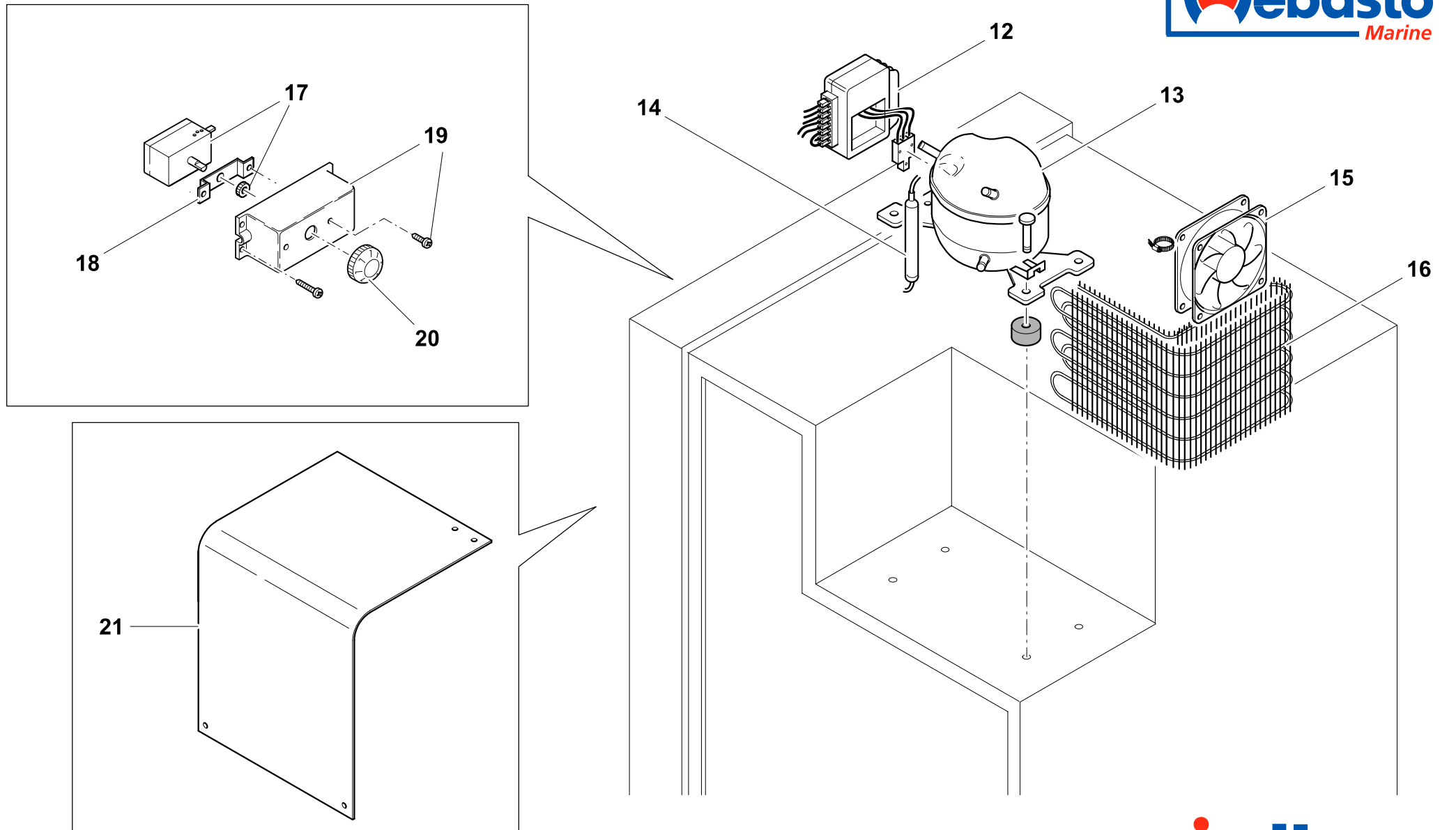
CR 90 FREEZER INOX - COOLING UNIT
